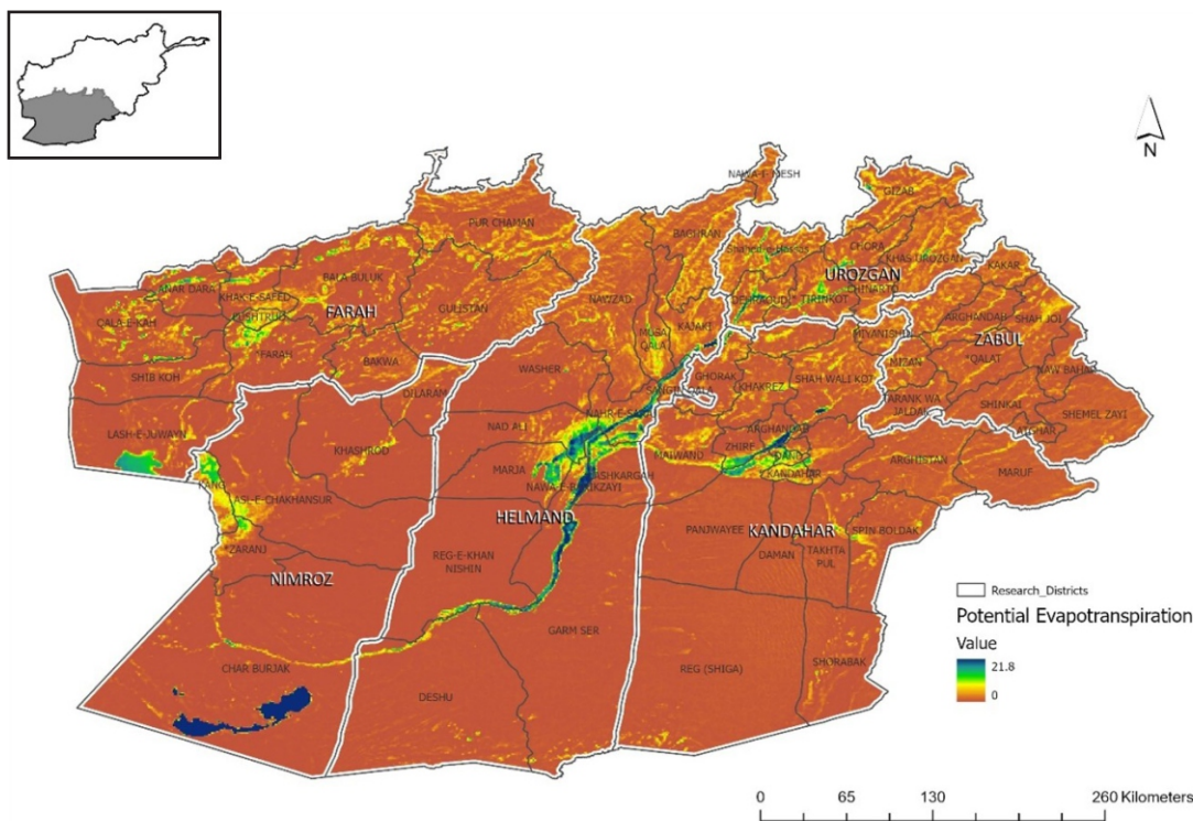
Figure 20 Potential Evapotranspiration, Research Area, 2018 - 2023, (source: authors)
